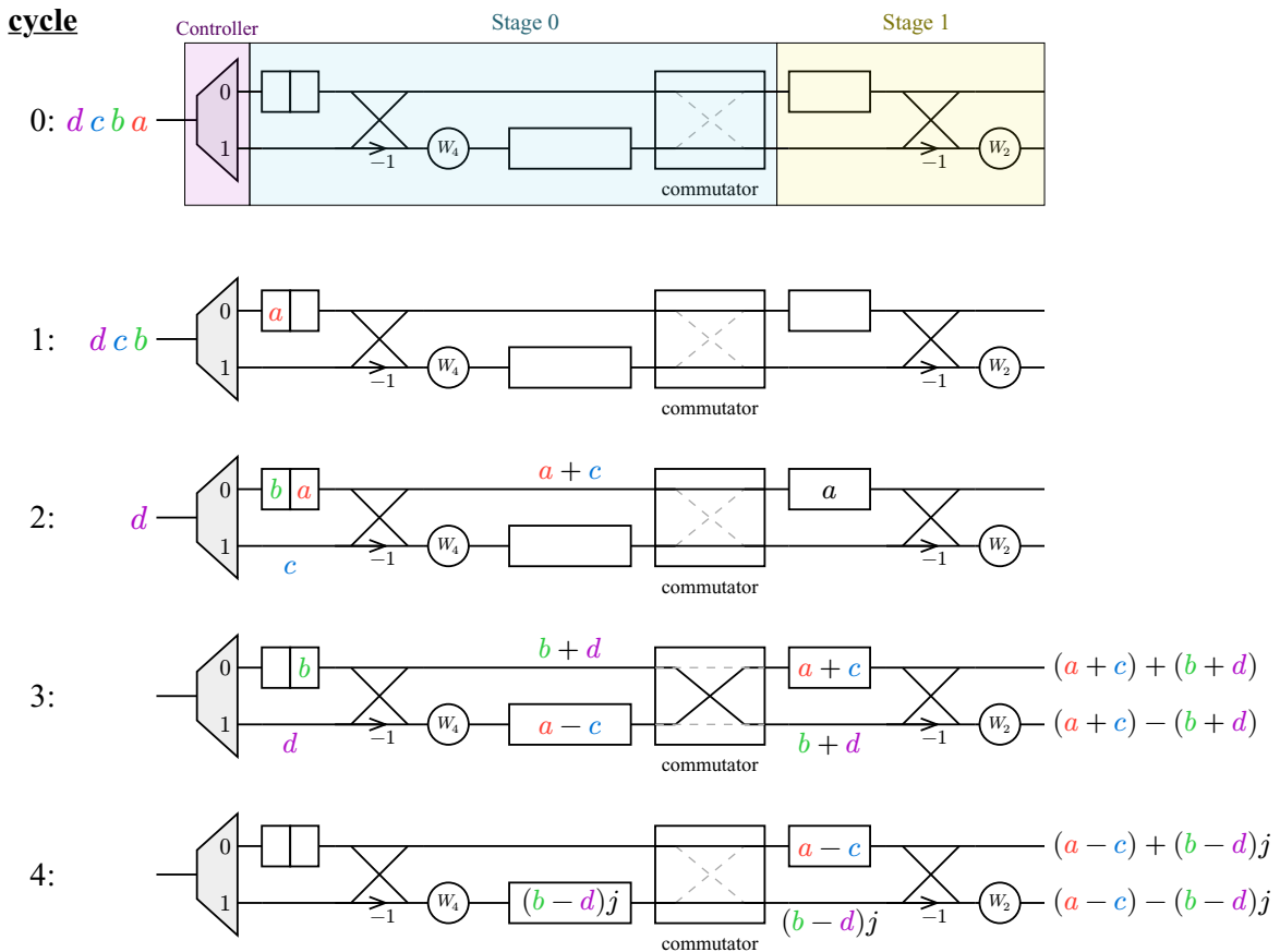
Figure 3.7: Steps in R2MDC algorithm for 4 point case
